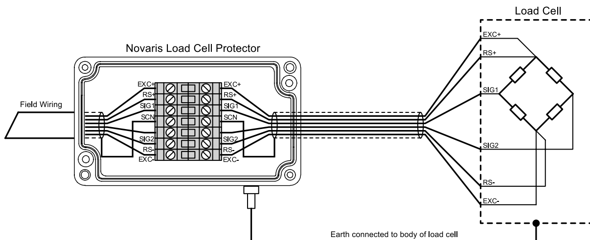
Figure 3. Installation of Load Cell Protector
