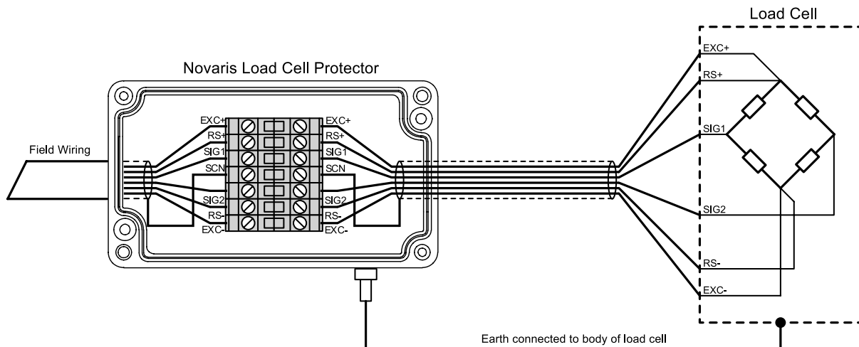
Figure 3. Installation of Load Cell Protector
