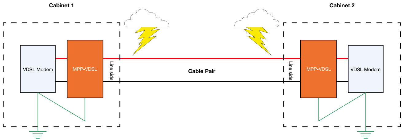
Figure 3. Connections for MPP-VDSL
