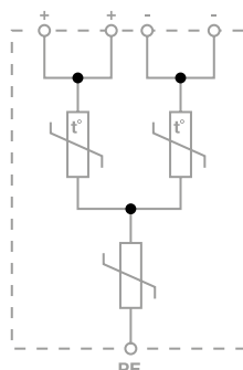
Figure 7. DC PV Configuration
