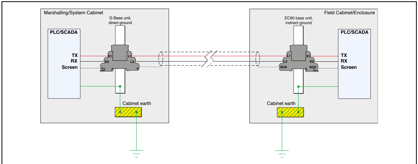
Figure 5. Example Showing Correct Orientation of SPD Connections with Single Screen Ground via SL36-G
