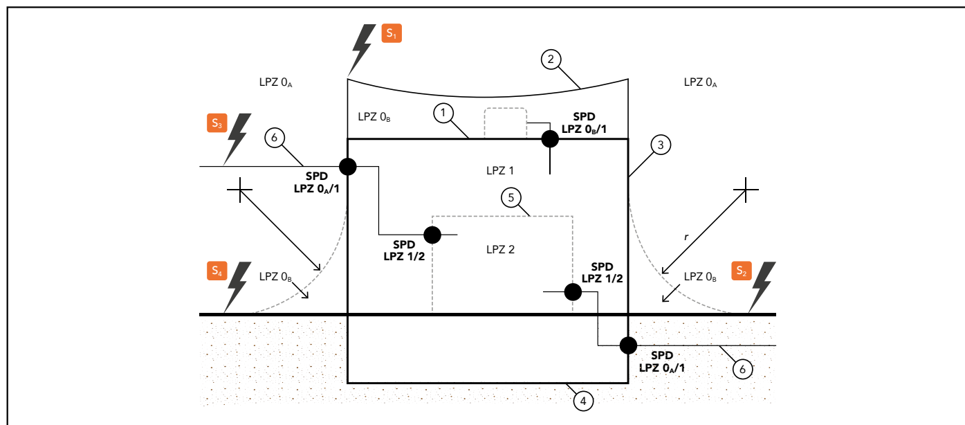
Figure 2. Lightning Protection Zones
