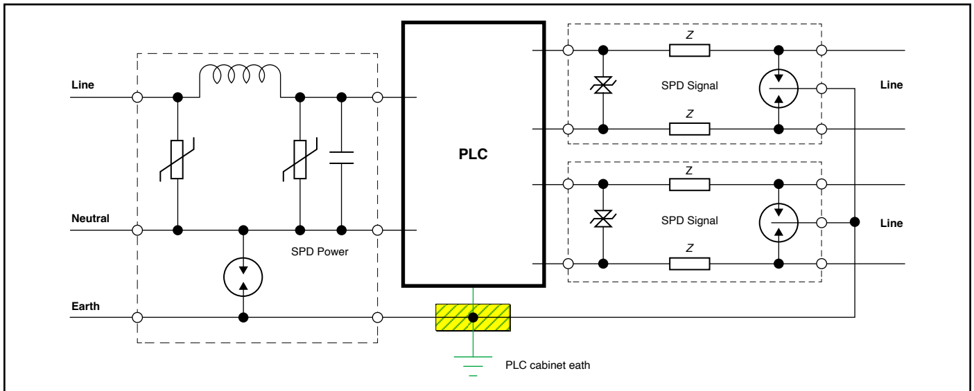
Figure 4. Common Earthing
