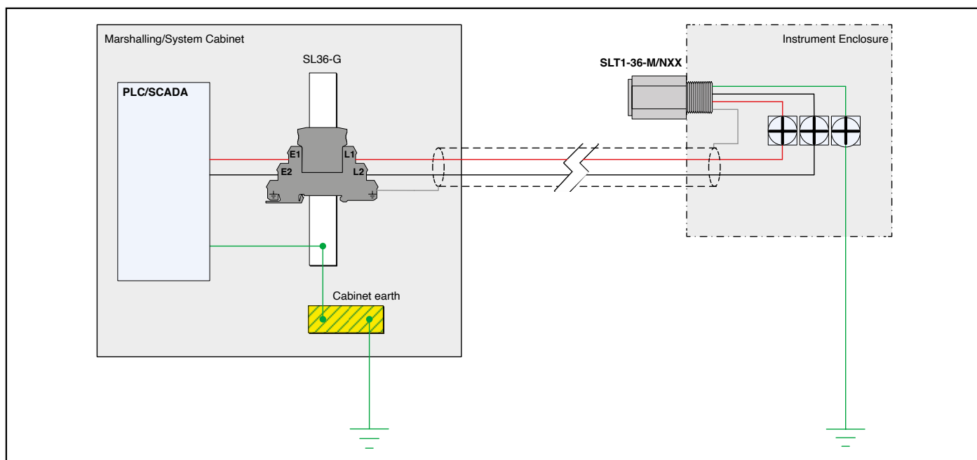
Figure 8. Surge Protection for Analogue and Digital I/O 2-Wire
