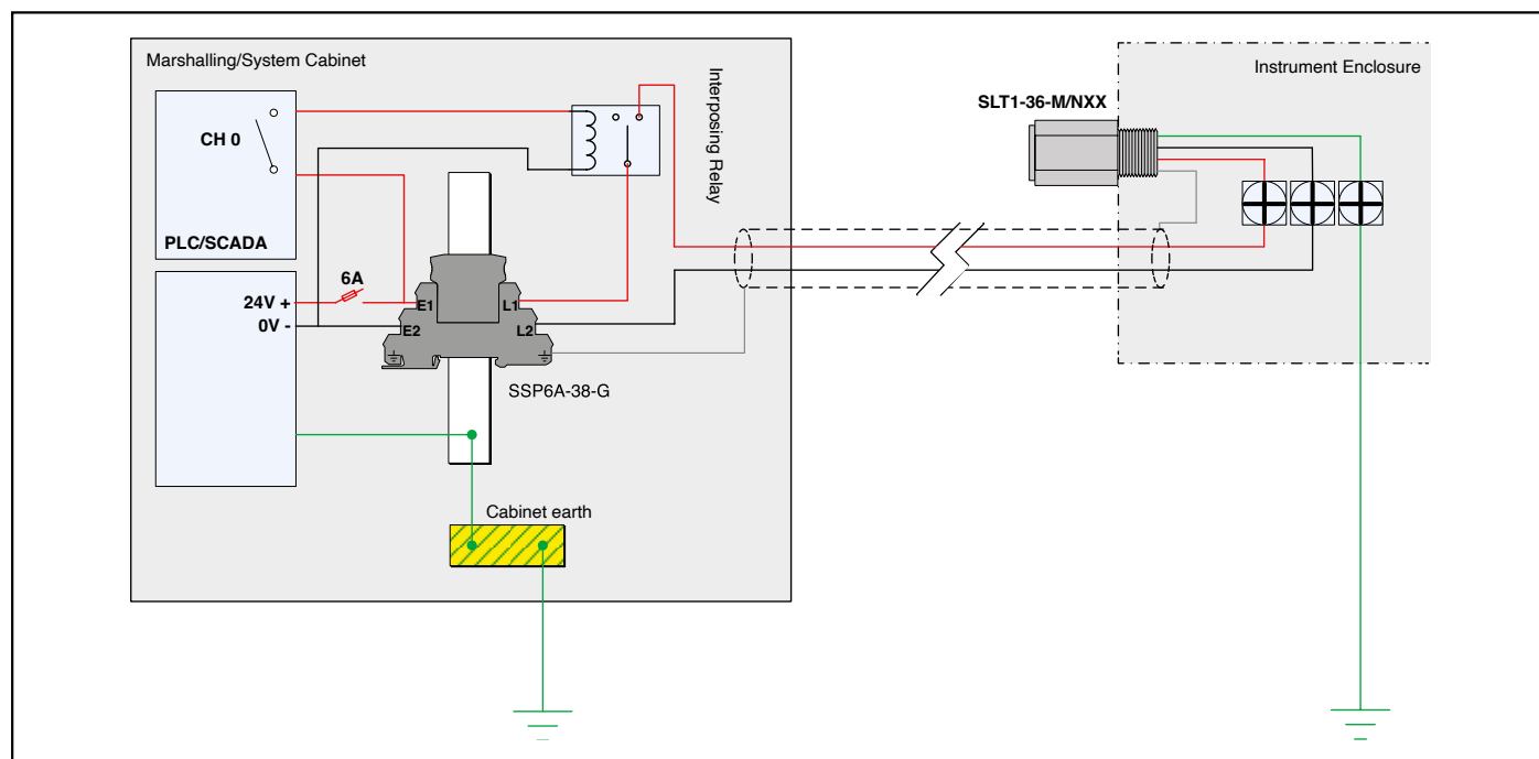
Figure 11. Surge Protection for I/O with Interposing Relay
