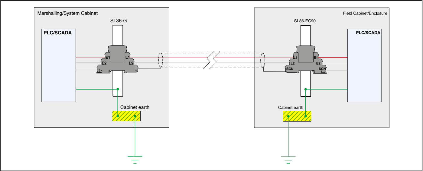
Figure 17. Surge Protection for RS232
