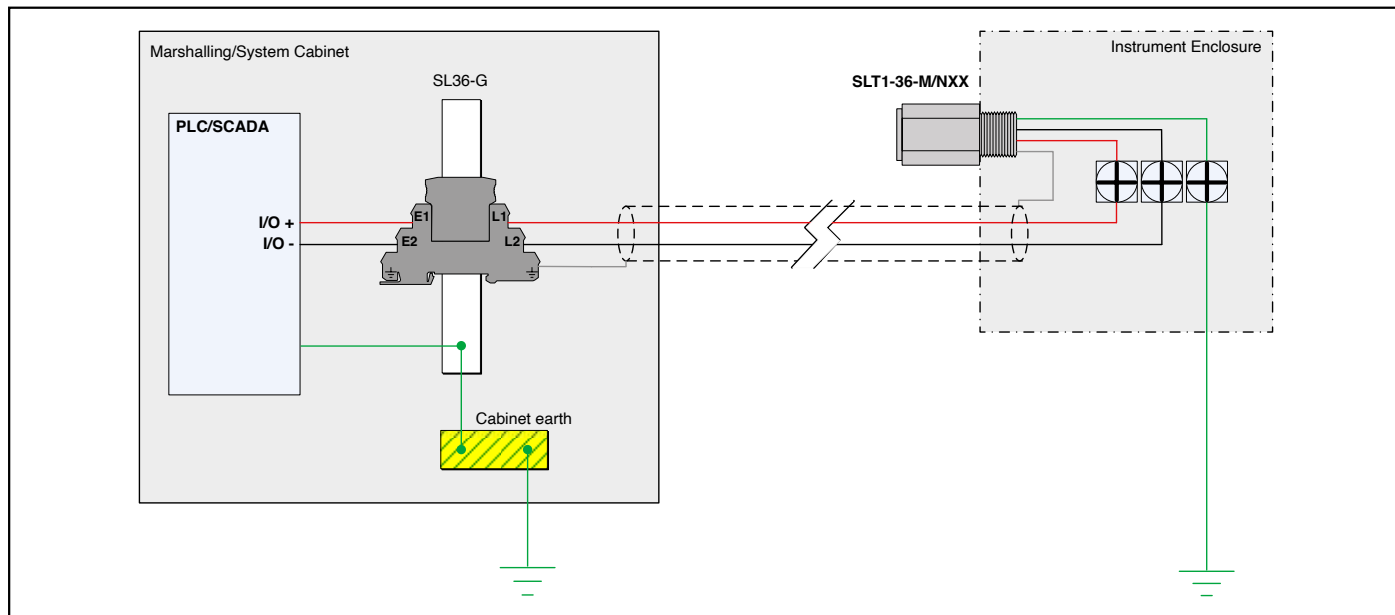
Figure 13. Surge protection for combined 4-20mA & HART
