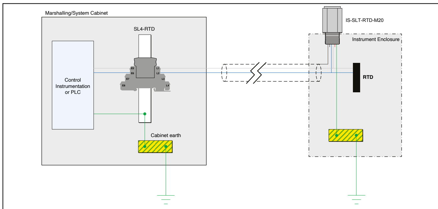
Figure 14. Surge Protection Wiring for a 2 Wire RTD
