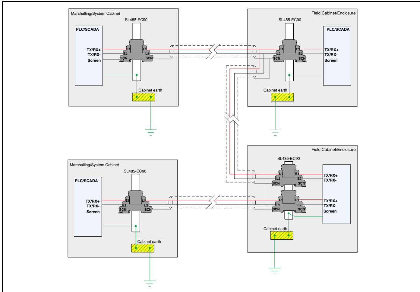
Figure 19. Surge Protection for Multidrop RS485
