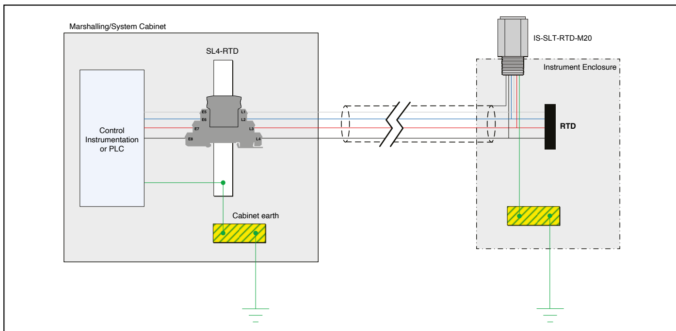
Figure 16. Surge Protection Wiring for a 4 Wire RTD
