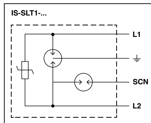
Figure 7. Example of Isolated Screen Connection for Field SPD
