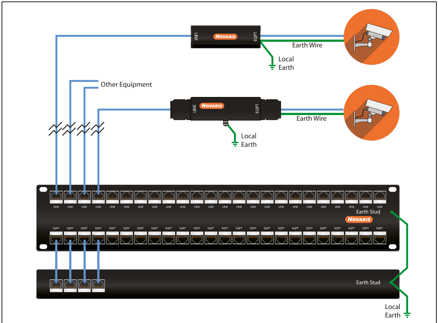
Figure 21. Surge Protection for Ethernet
