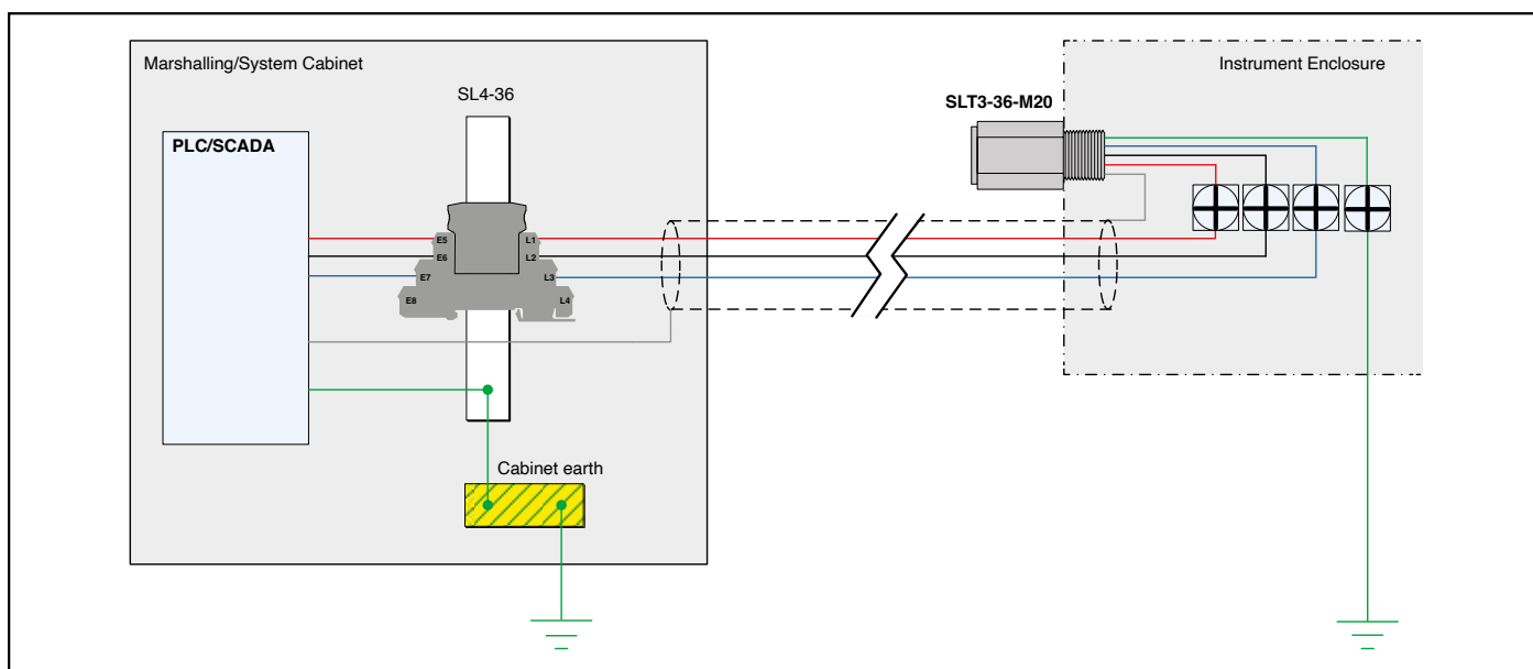
Figure 9. Surge Protection for Analogue and Digital I/O 3-Wire
