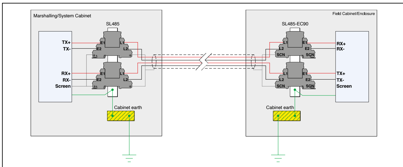
Figure 20. Surge Protection for RS422
