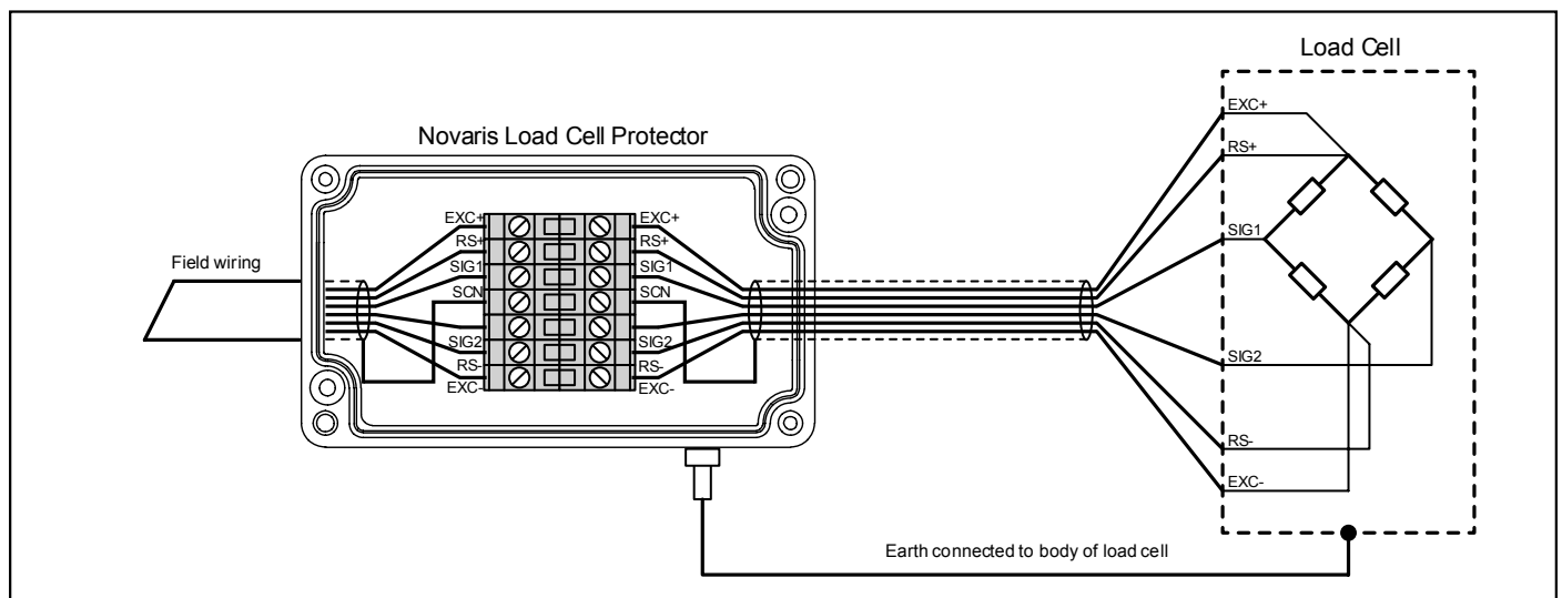
Figure 25. LCP Wiring Schematic
