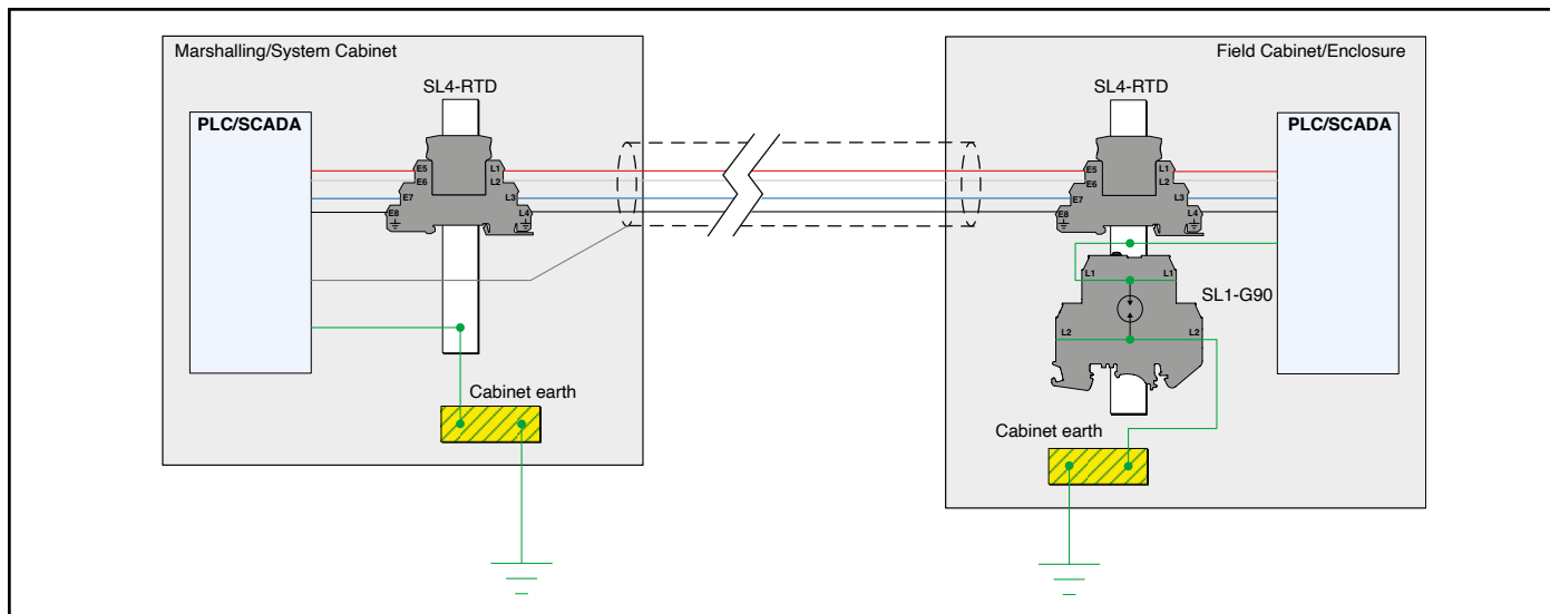
Figure 6. Use of SL1-G90 with an SL4 (Ensure Field Side DIN rail is Not Earthed Other than via the SL1-G90)
