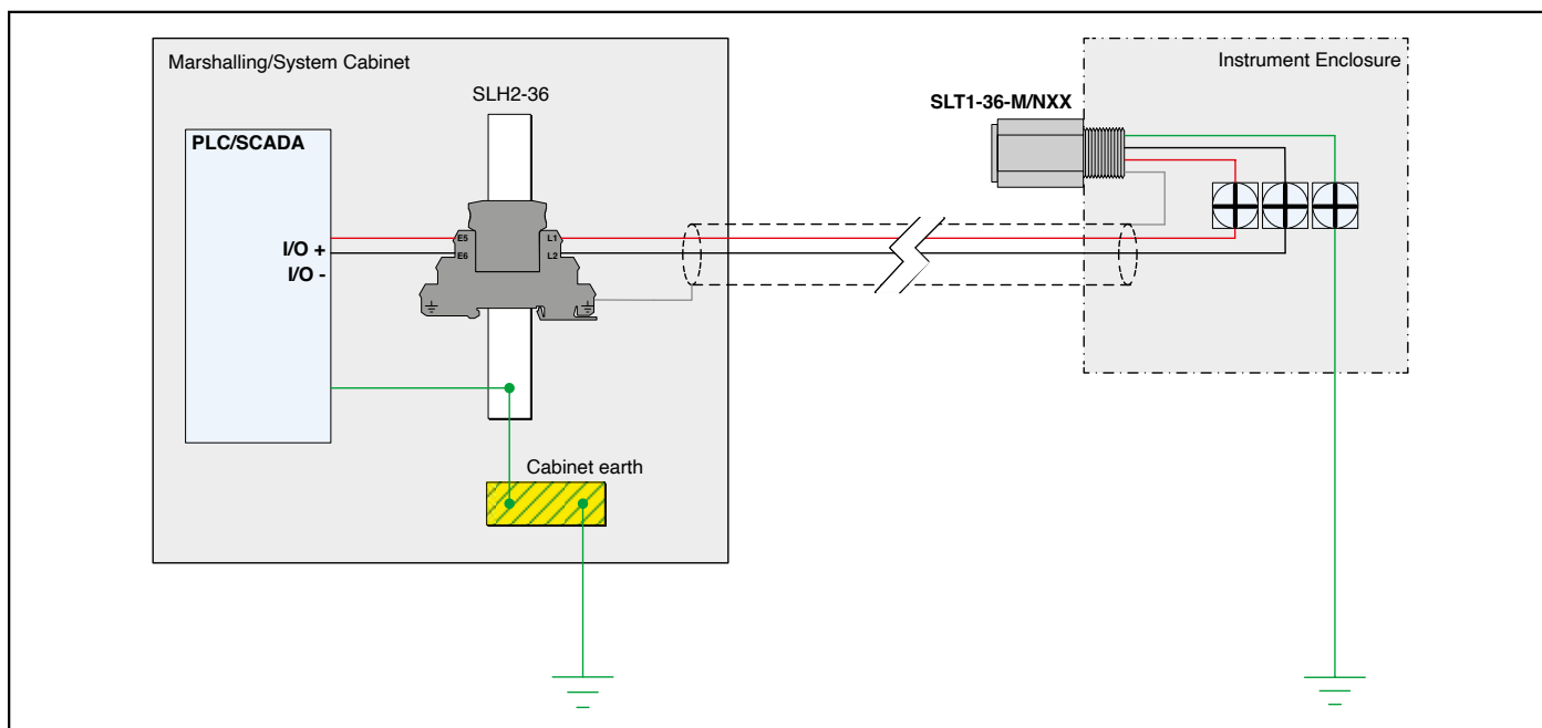
Figure 10. Surge Protection for I/O up to 2.5A
