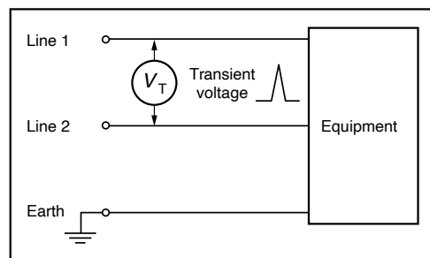
Figure 1b. Transverse / Differential Mode Transient
