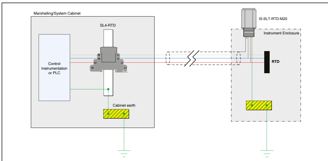
Figure 15. Surge Protection Wiring for a 3 Wire RTD
