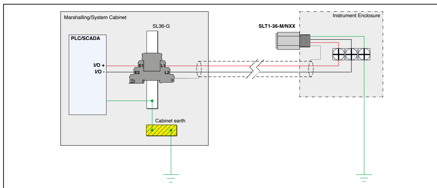
Figure 12. Surge Protection for a 4-20mA Instrument Loop
