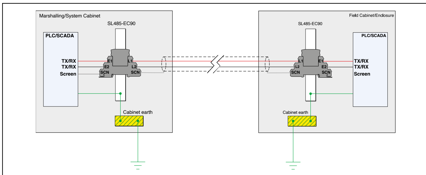
Figure 18. Surge Protection for RS485
