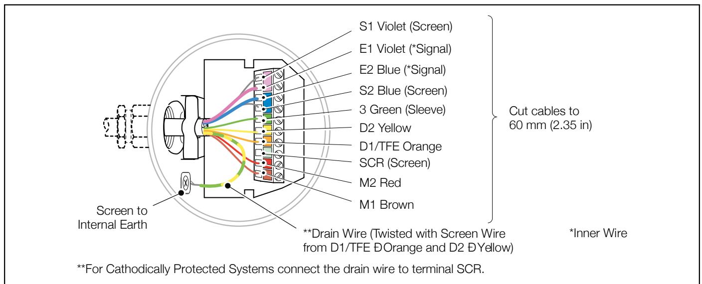
Figure 22. ABB WaterMaster sensor connection schematic, courtesy of ABB
