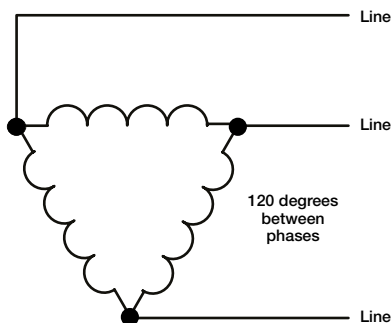
Figure 7. 3-Phase Delta Connection
