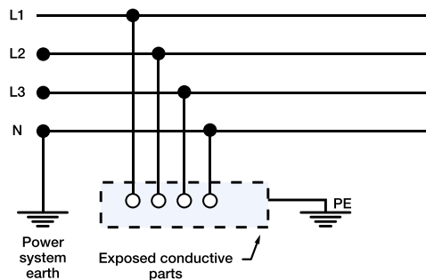
Figure 4. TT System Schematic
