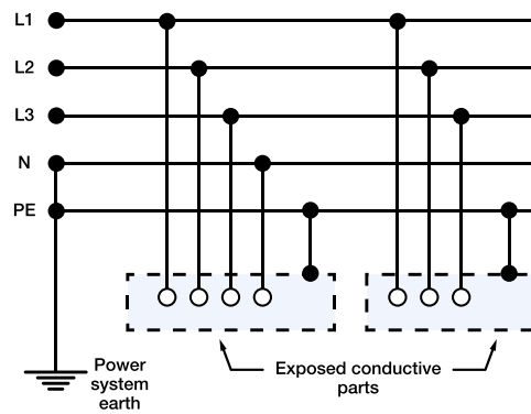
Figure 1. TN-S System Schematic
