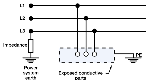
Figure 5. IT System Schematic
