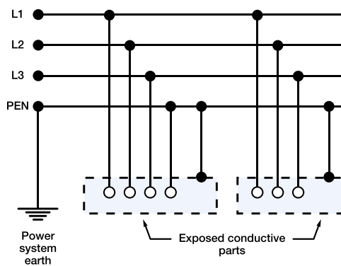
Figure 2. TN-C System Schematic
