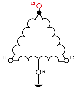
Figure 10. Hi-Leg Delta Connection Diagram Showing 2-Phase Connections via L1 and L2
