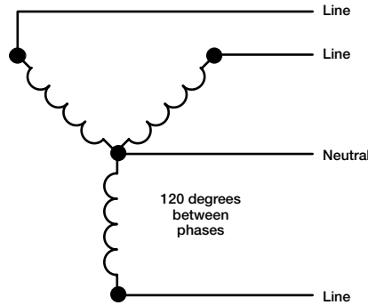
Figure 8. 4 Wire Star Connection with Neutral Conductor
