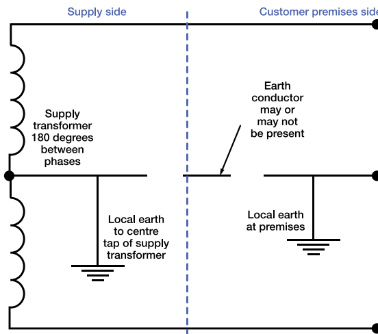
Figure 11. Two-Phase Supply Connection Diagram
