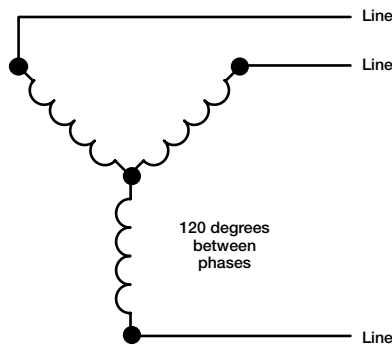
Figure 9. 4 Star Connection with 3 Wires
