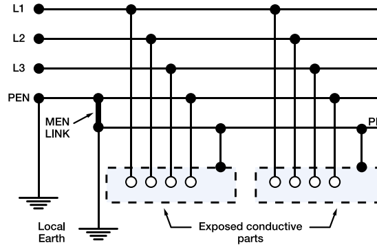
Figure 3. TN-C-S System Schematic
